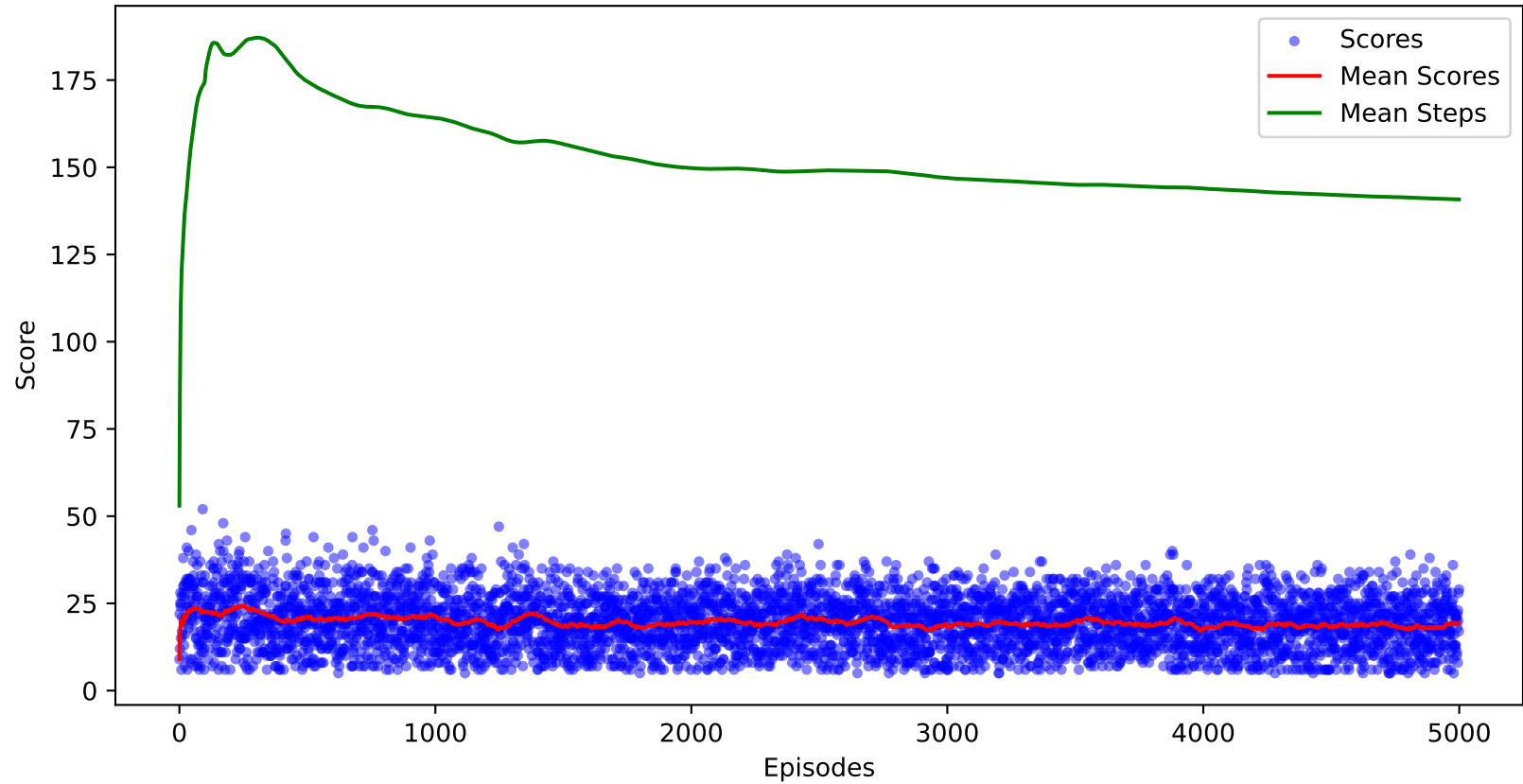
Training Progress
